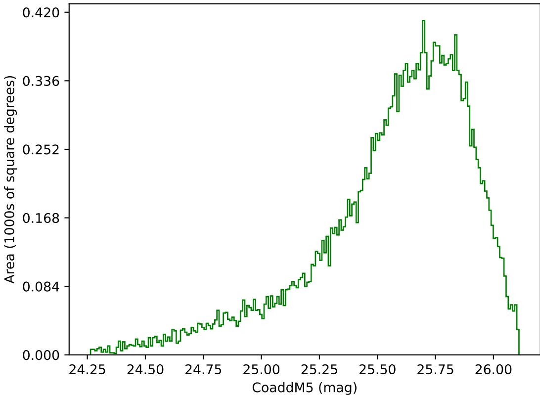
ddf_loaded_half_fl15_v3.4_10yrs Yr 1 g band: CoaddM5
