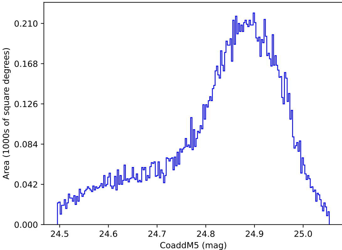
ddf_loaded_half_fl15_v3.4_10yrs WFD y band: CoaddM5
