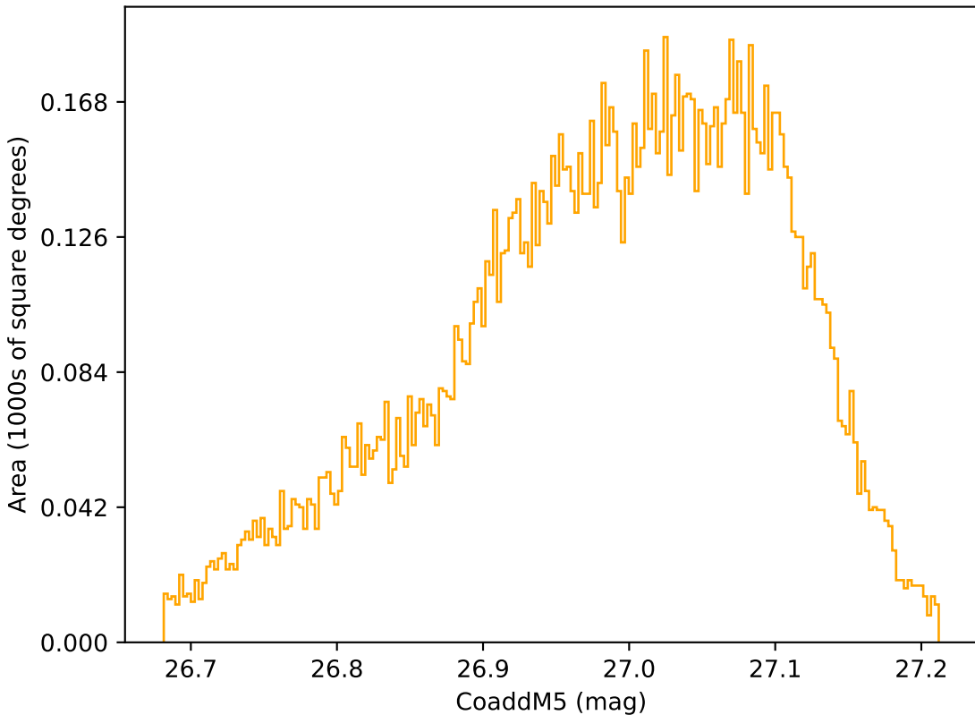
ddf_loaded_half_fl15_v3.4_10yrs WFD r band: CoaddM5
