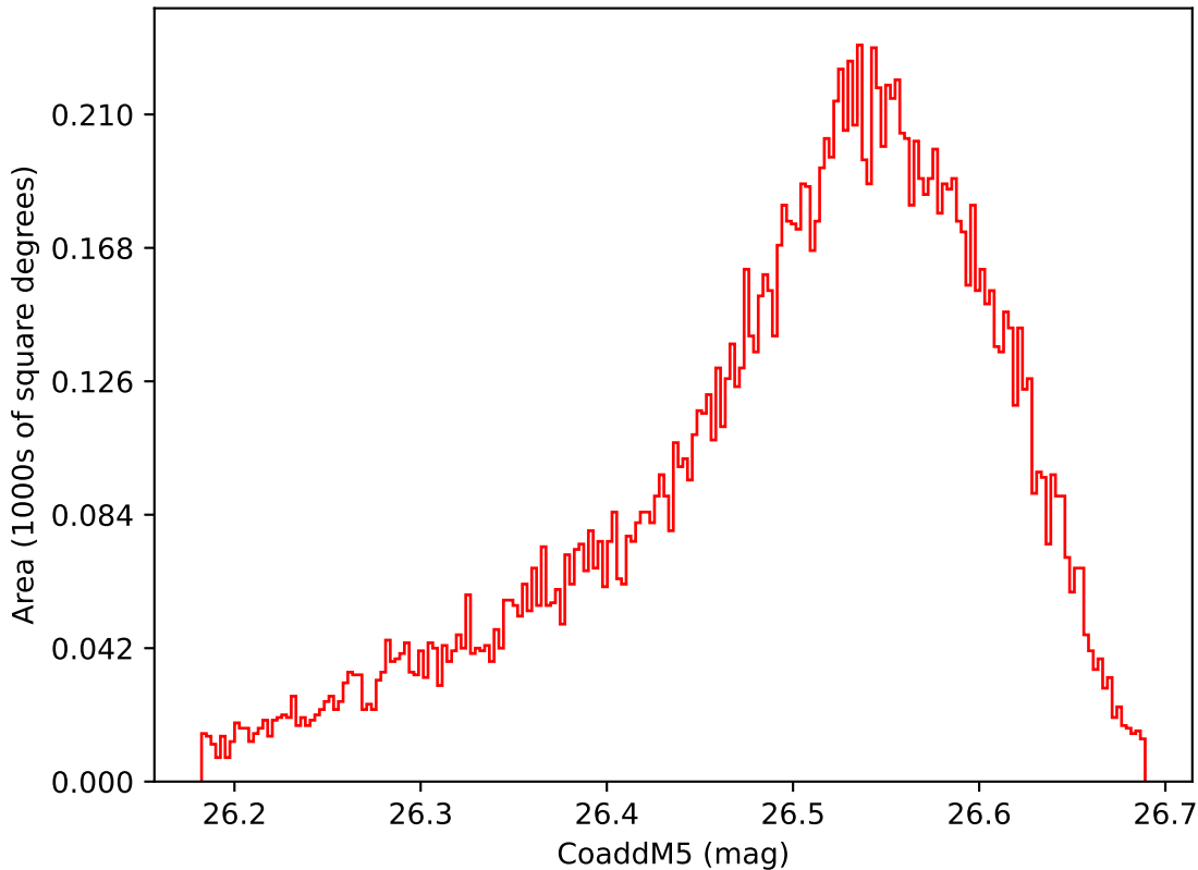
ddf_loaded_half_fl15_v3.4_10yrs WFD i band: CoaddM5
