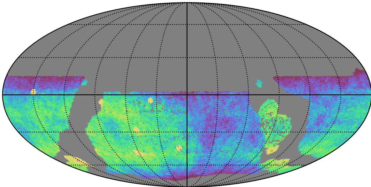
ddf_loaded_half_fl15_v3.4_10yrs WFD g band: CoaddM5
