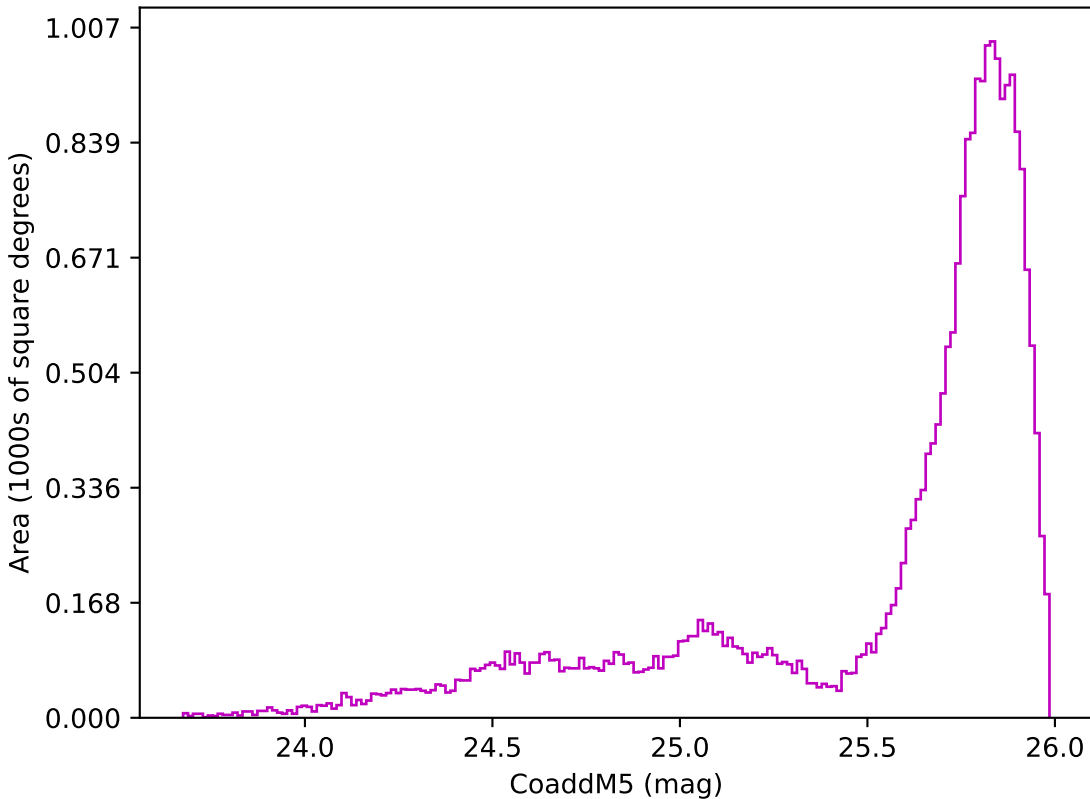
ddf_loaded_half_fl15_v3.4_10yrs All sky z band: CoaddM5
