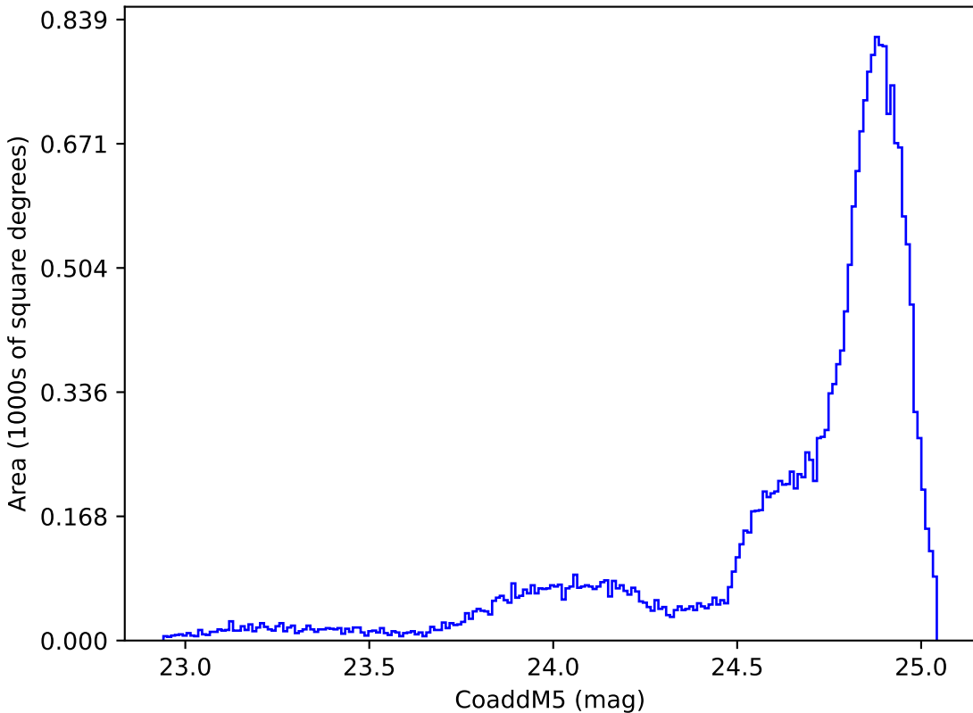
ddf_loaded_half_fl15_v3.4_10yrs All sky y band: CoaddM5
