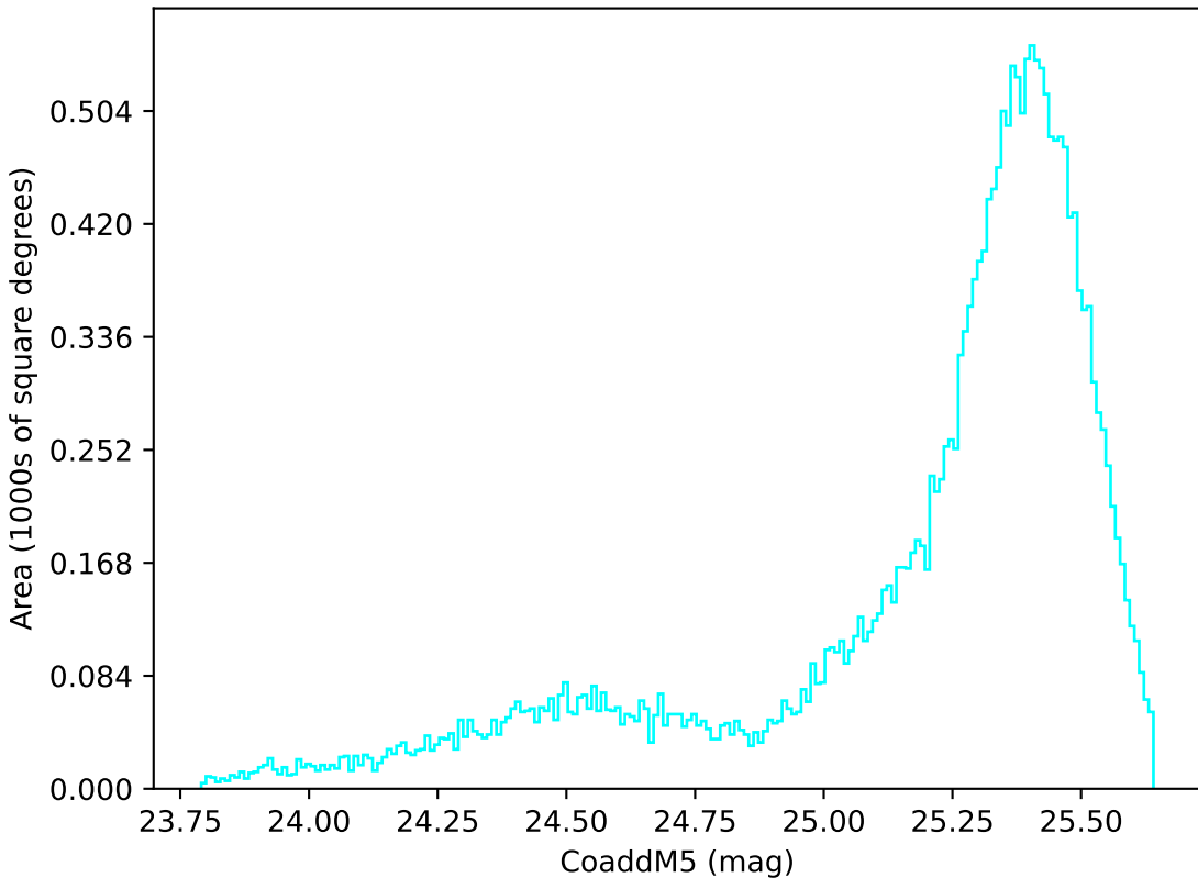
ddf_loaded_half_fl15_v3.4_10yrs All sky u band: CoaddM5
