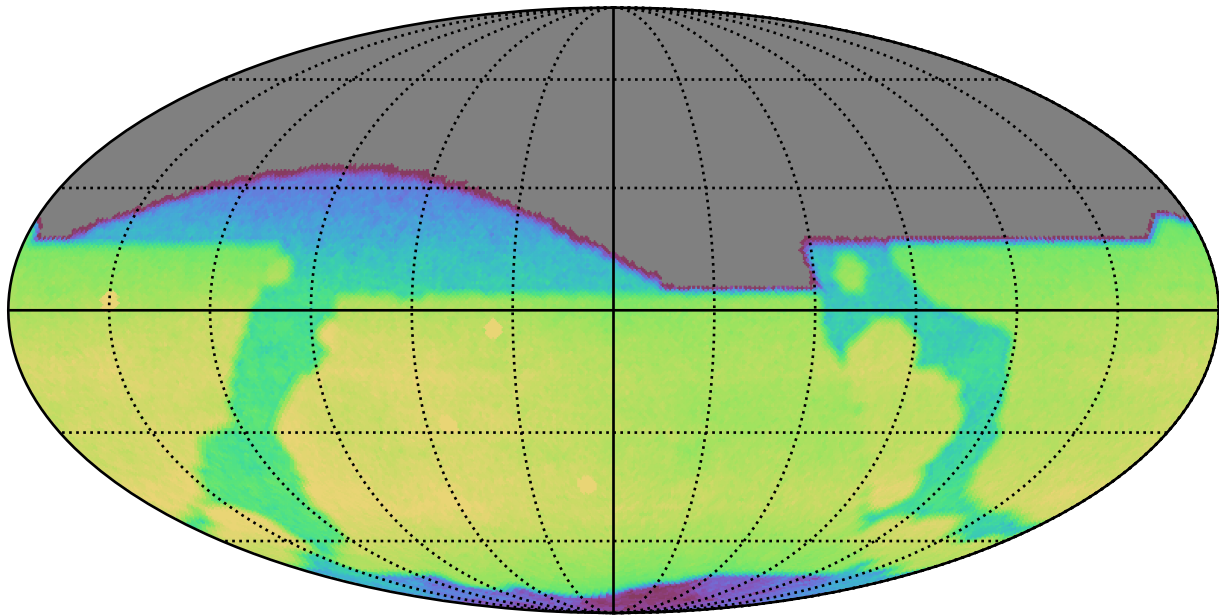
ddf_loaded_half_fl15_v3.4_10yrs All sky r band: CoaddM5
