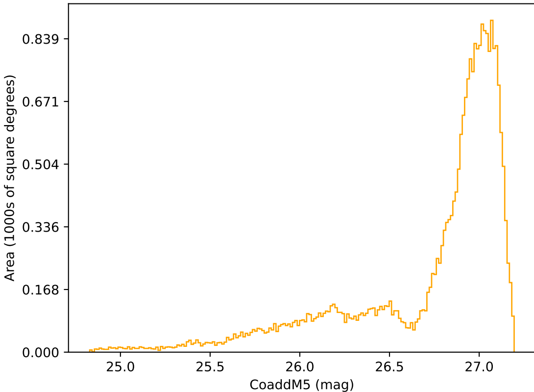
ddf_loaded_half_fl15_v3.4_10yrs All sky r band: CoaddM5
