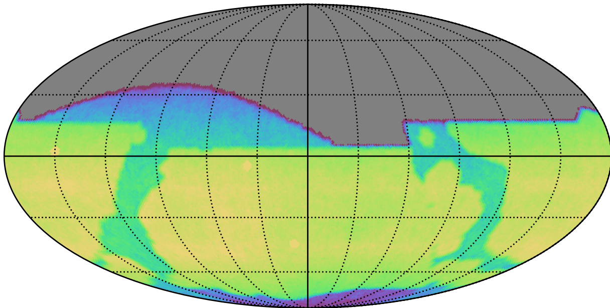
ddf_loaded_half_fl15_v3.4_10yrs All sky i band: CoaddM5
