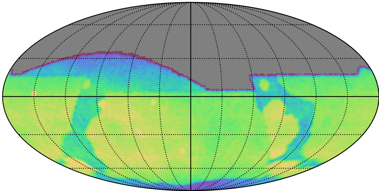
ddf_loaded_half_fl15_v3.4_10yrs All sky g band: CoaddM5
