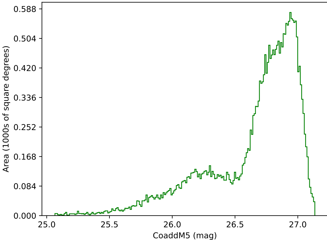
ddf_loaded_half_fl15_v3.4_10yrs All sky g band: CoaddM5
