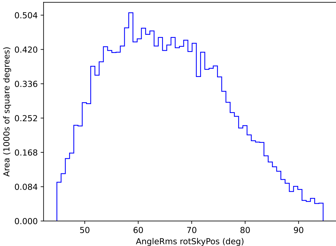
ddf_loaded_half_fl15_v3.4_10yrs WFD u band: AngleRms rotSkyPos
