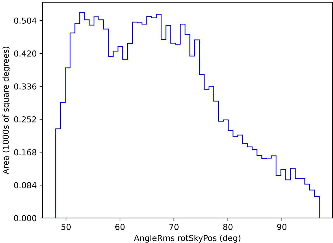
ddf_loaded_half_fl15_v3.4_10yrs WFD r band: AngleRms rotSkyPos
