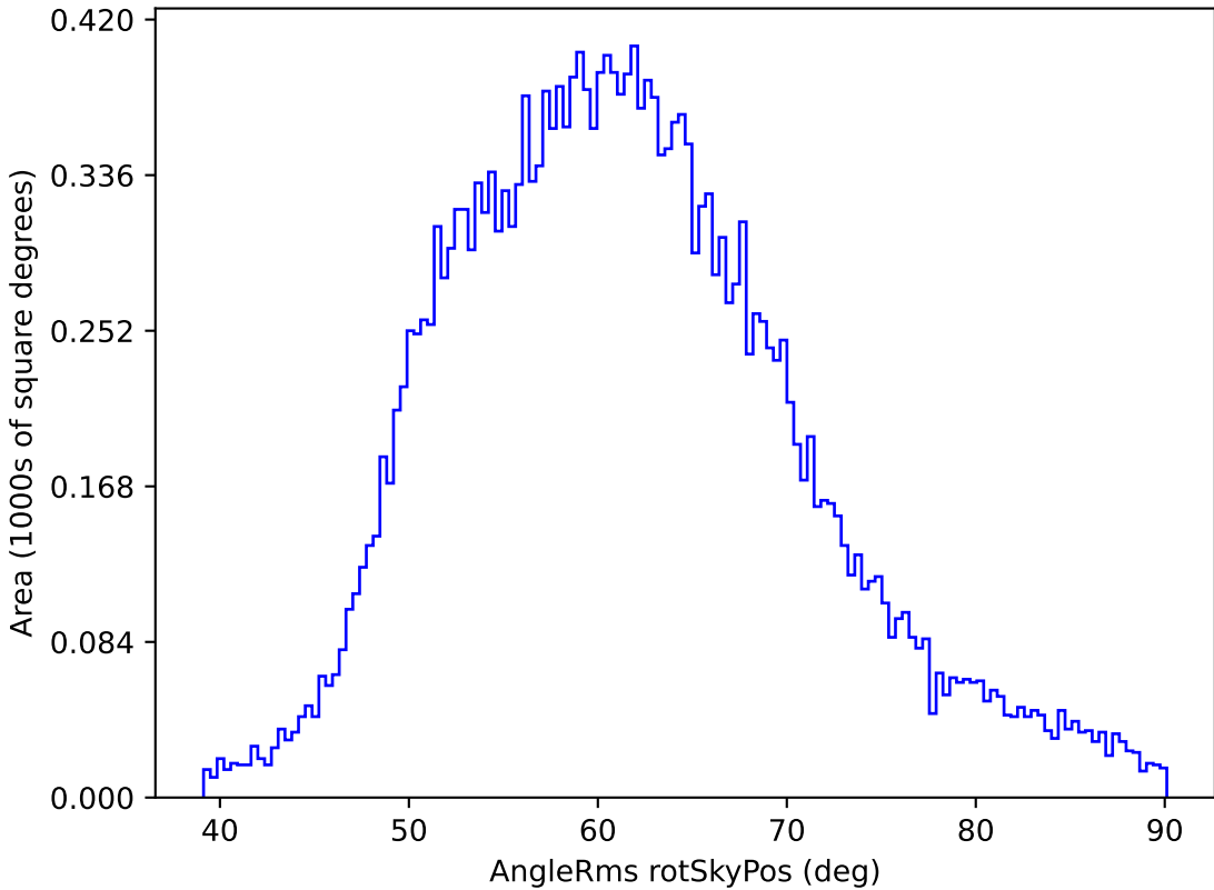
ddf_loaded_half_fl15_v3.4_10yrs All sky y band: AngleRms rotSkyPos
