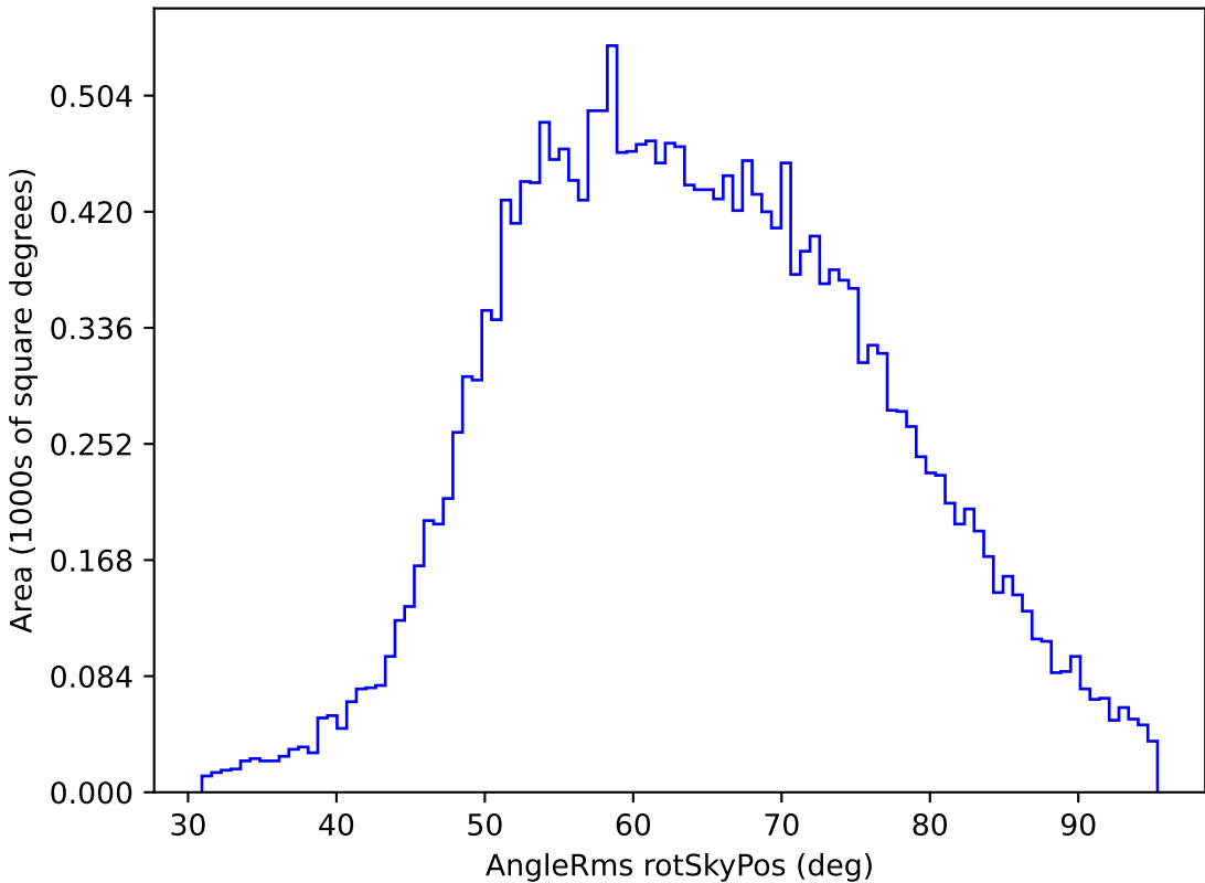
ddf_loaded_half_fl15_v3.4_10yrs All sky u band: AngleRms rotSkyPos
