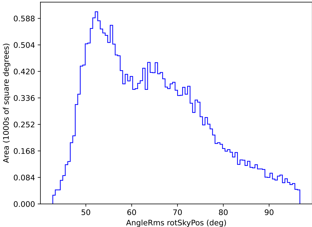
ddf_loaded_half_fl15_v3.4_10yrs All sky r band: AngleRms rotSkyPos
