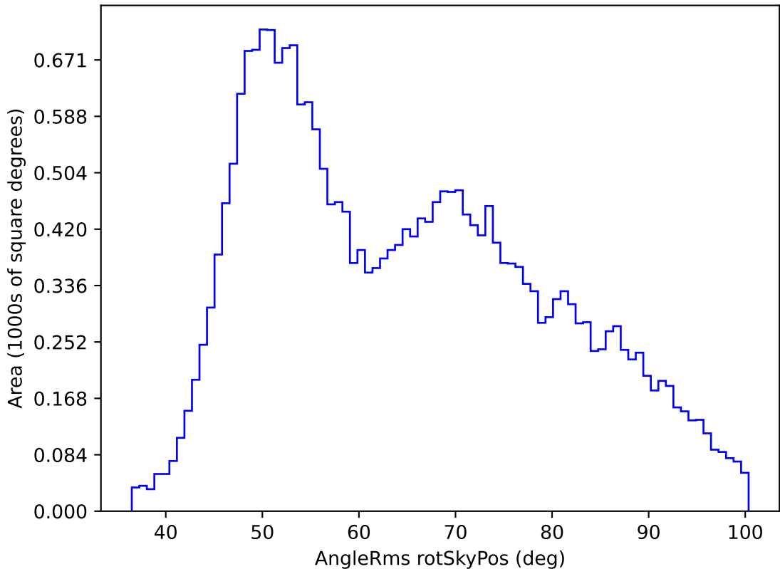
ddf_loaded_half_fl15_v3.4_10yrs All sky g band: AngleRms rotSkyPos
