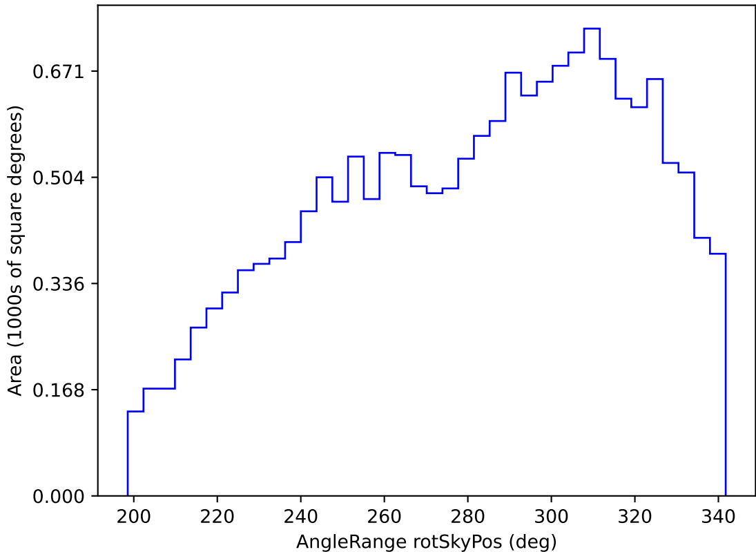
ddf_loaded_half_fl15_v3.4_10yrs WFD z band: AngleRange rotSkyPos
