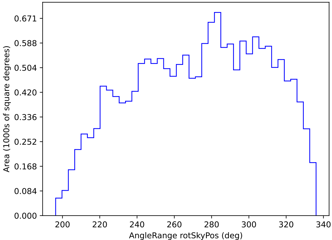
ddf_loaded_half_fl15_v3.4_10yrs WFD y band: AngleRange rotSkyPos
