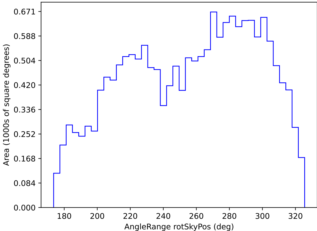
ddf_loaded_half_fl15_v3.4_10yrs WFD u band: AngleRange rotSkyPos
