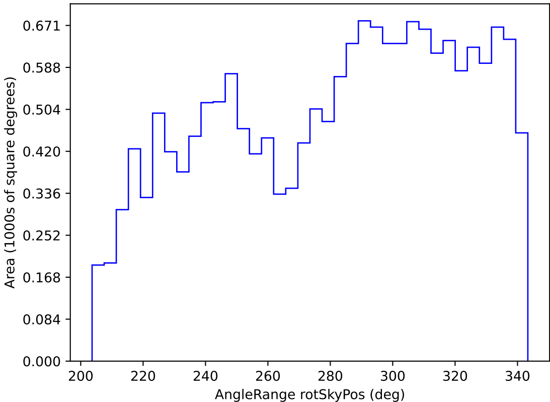
ddf_loaded_half_fl15_v3.4_10yrs WFD r band: AngleRange rotSkyPos
