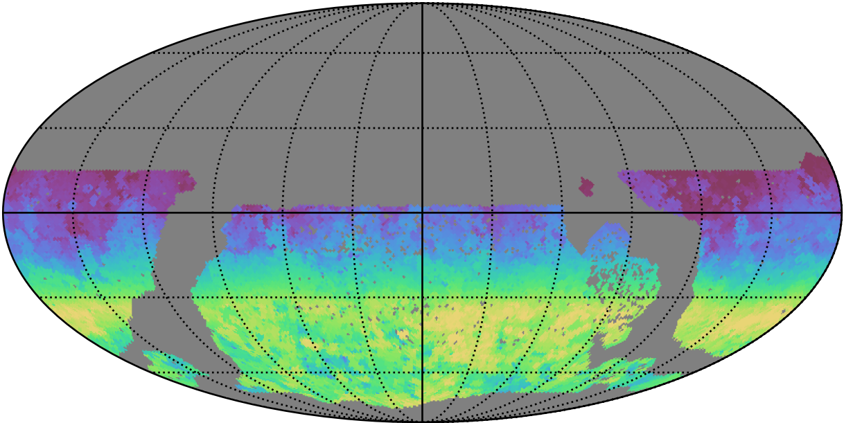
ddf_loaded_half_fl15_v3.4_10yrs WFD i band: AngleRange rotSkyPos
