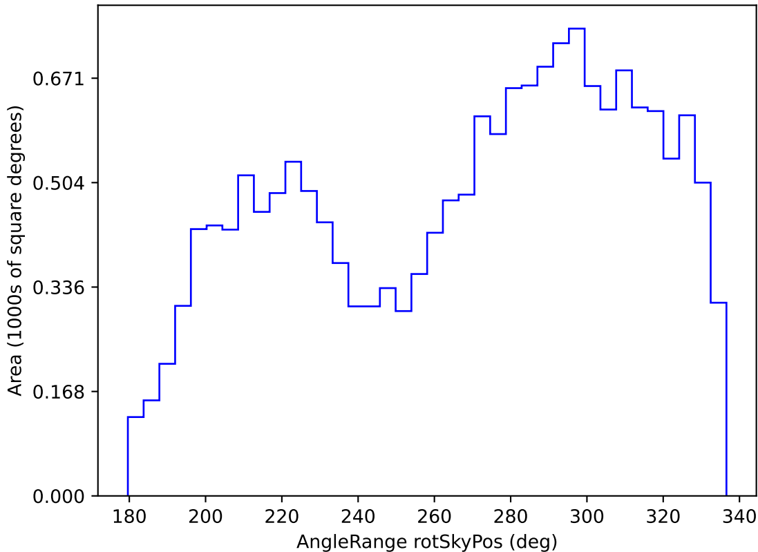
ddf_loaded_half_fl15_v3.4_10yrs WFD g band: AngleRange rotSkyPos
