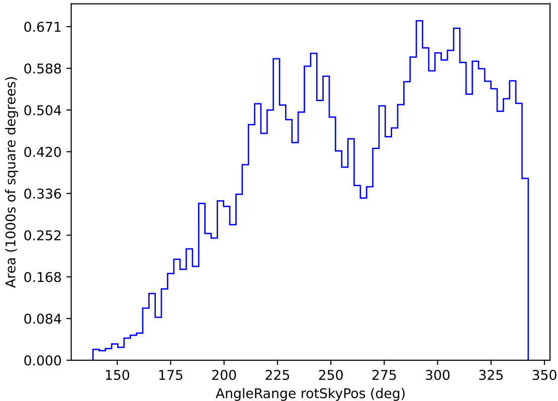
ddf_loaded_half_fl15_v3.4_10yrs All sky r band: AngleRange rotSkyPos
