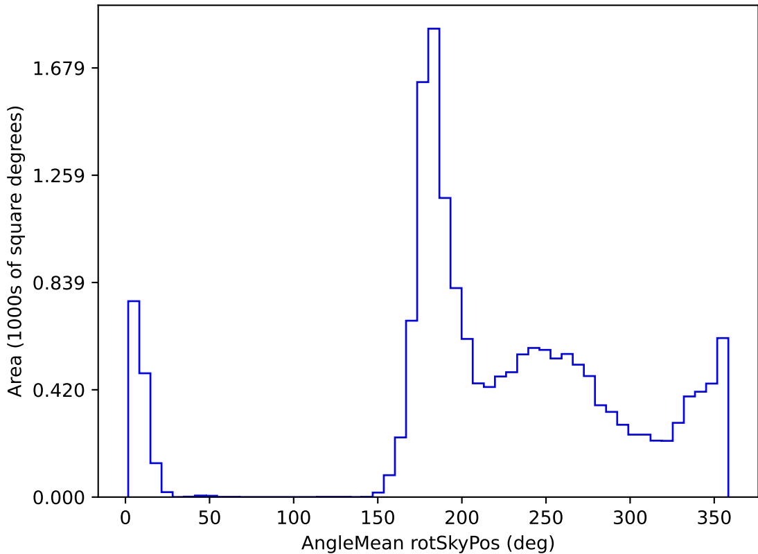
ddf_loaded_half_fl15_v3.4_10yrs WFD y band: AngleMean rotSkyPos
