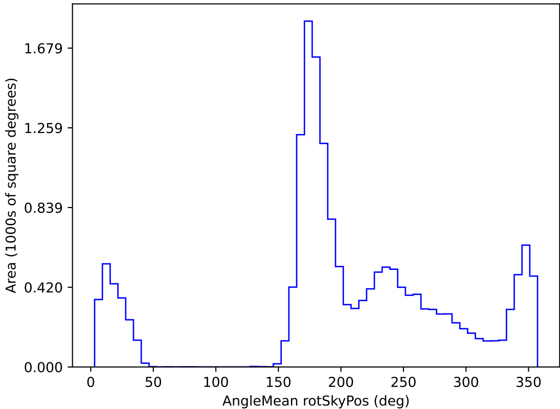
ddf_loaded_half_fl15_v3.4_10yrs WFD r band: AngleMean rotSkyPos
