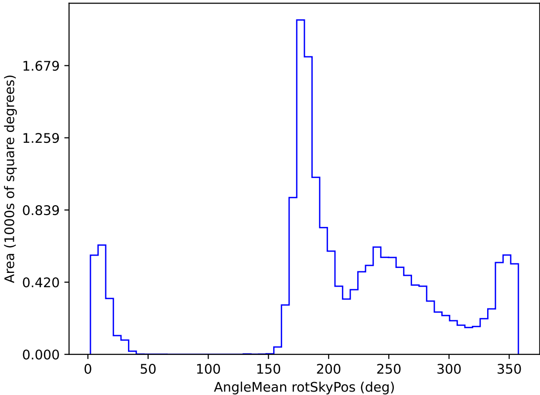
ddf_loaded_half_fl15_v3.4_10yrs WFD i band: AngleMean rotSkyPos
