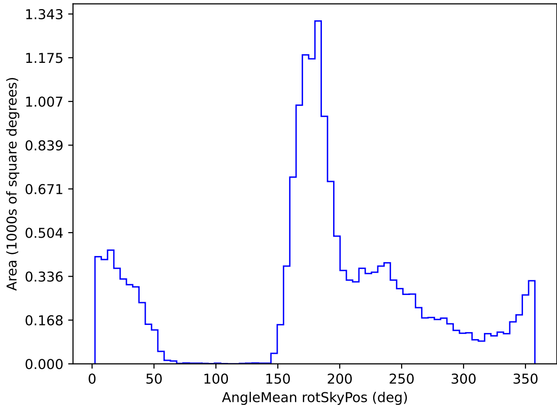
ddf_loaded_half_fl15_v3.4_10yrs WFD g band: AngleMean rotSkyPos
