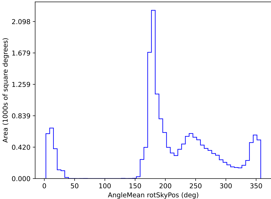
ddf_loaded_half_fl15_v3.4_10yrs WFD all bands: AngleMean rotSkyPos
