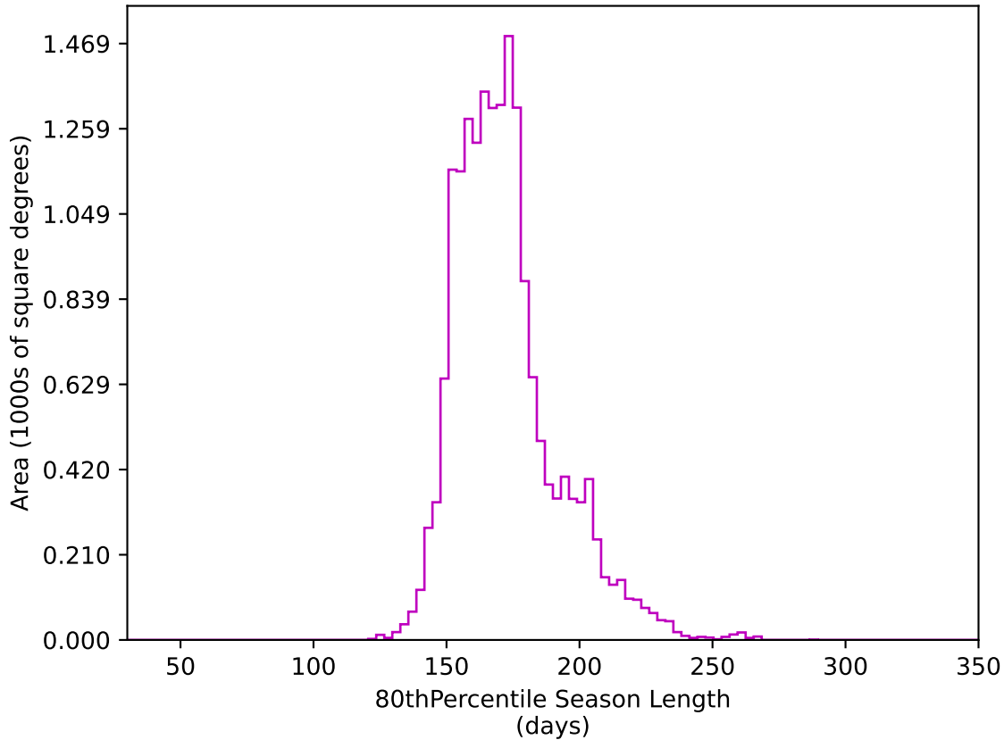
ddf_loaded_half_fl15_v3.4_10yrs WFD z band: 80thPercentile Season Length
