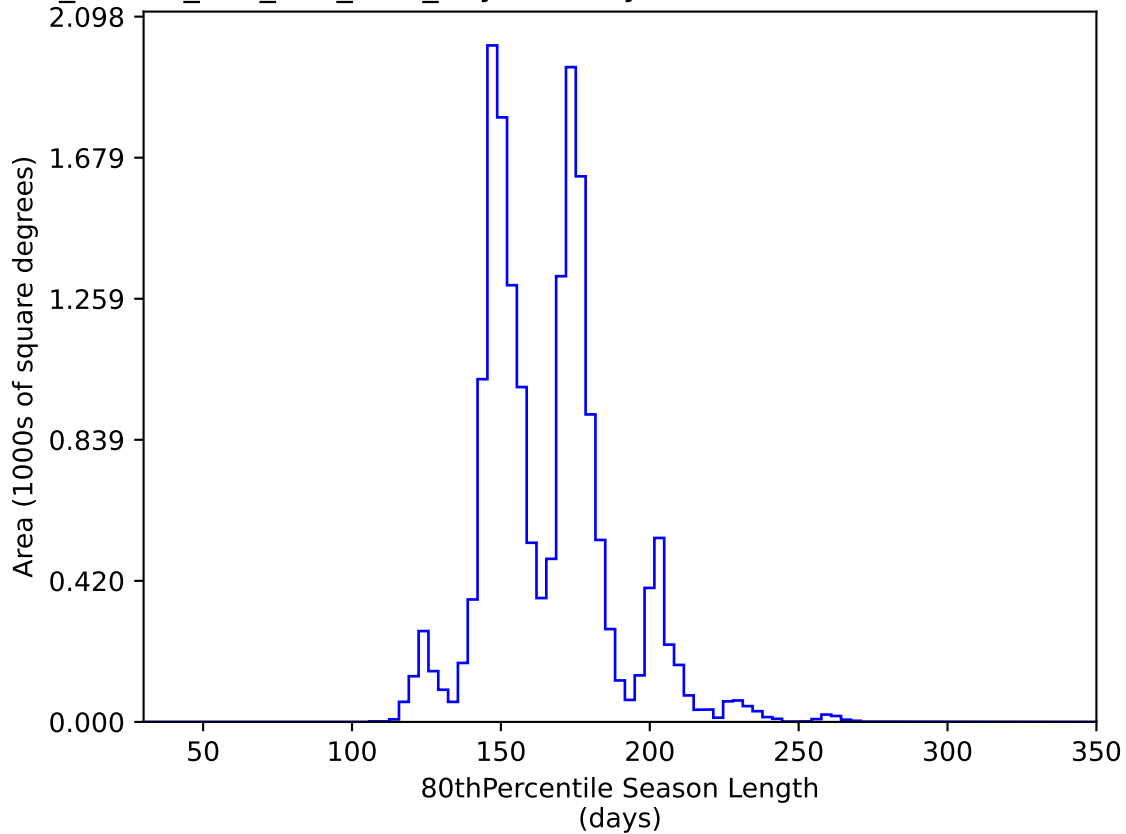
ddf_loaded_half_fl15_v3.4_10yrs WFD y band: 80thPercentile Season Length
