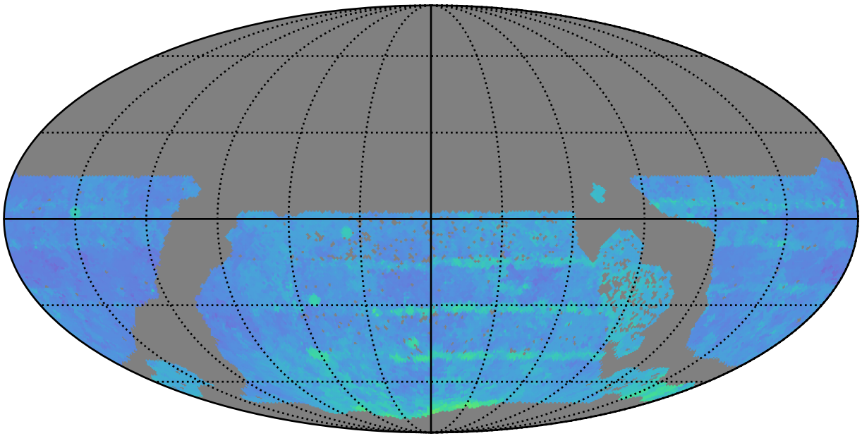
ddf_loaded_half_fl15_v3.4_10yrs WFD r band: 80thPercentile Season Length
