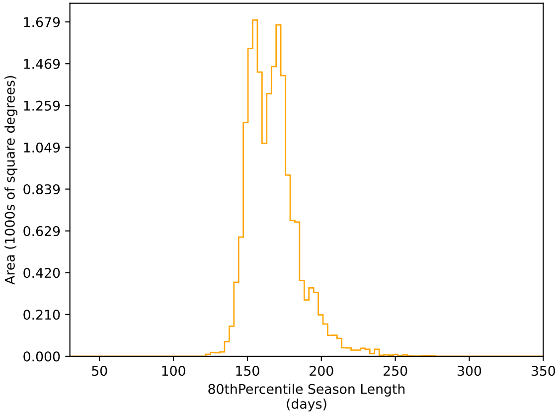
ddf_loaded_half_fl15_v3.4_10yrs WFD r band: 80thPercentile Season Length
