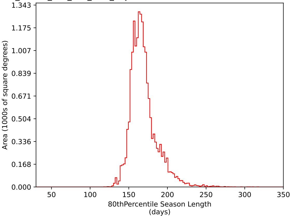
ddf_loaded_half_fl15_v3.4_10yrs WFD i band: 80thPercentile Season Length
