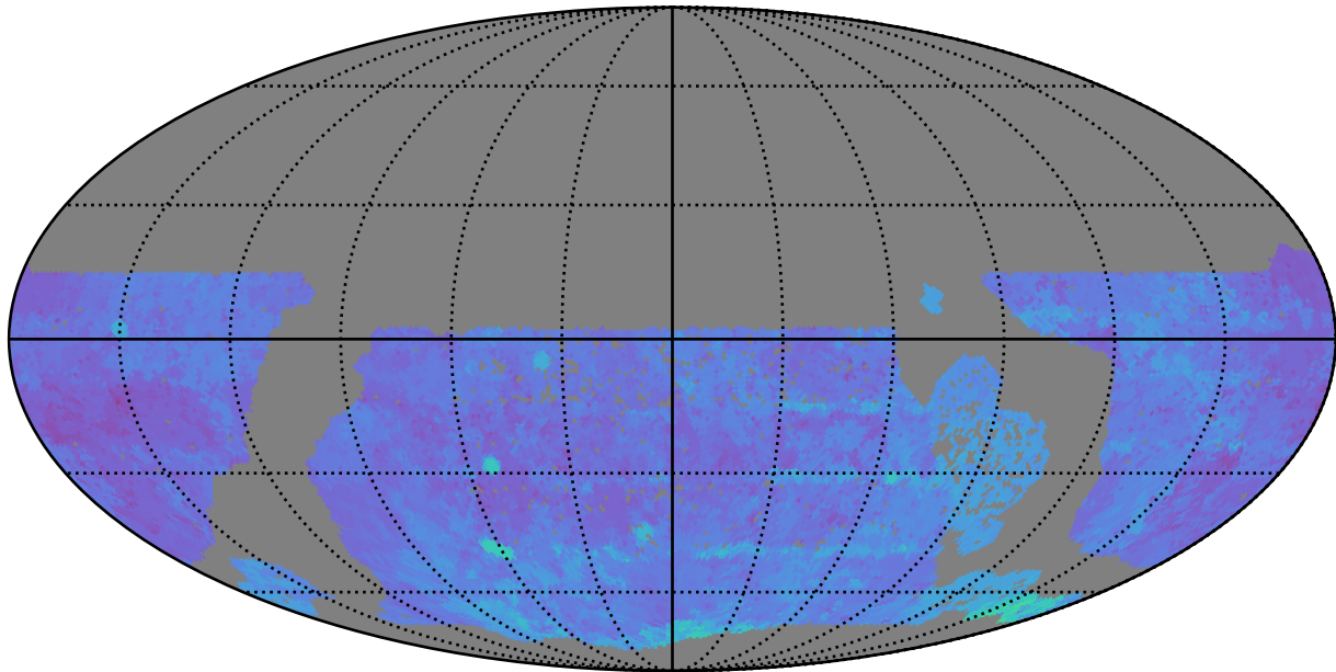
ddf_loaded_half_fl15_v3.4_10yrs WFD g band: 80thPercentile Season Length
