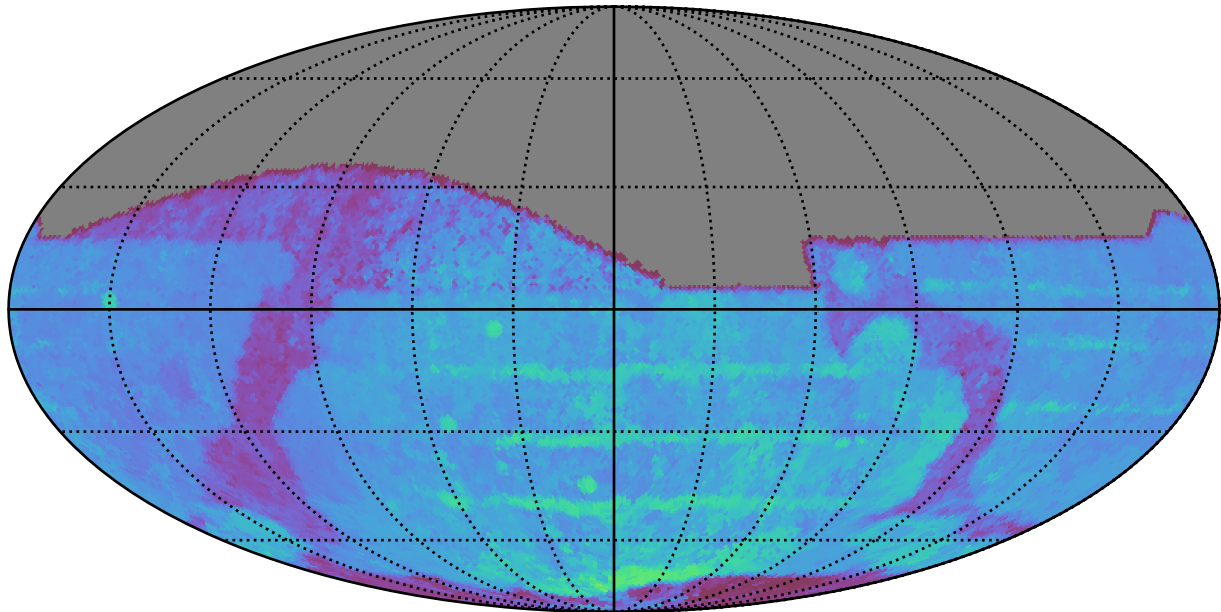
ddf_loaded_half_fl15_v3.4_10yrs All sky z band: 80thPercentile Season Length
