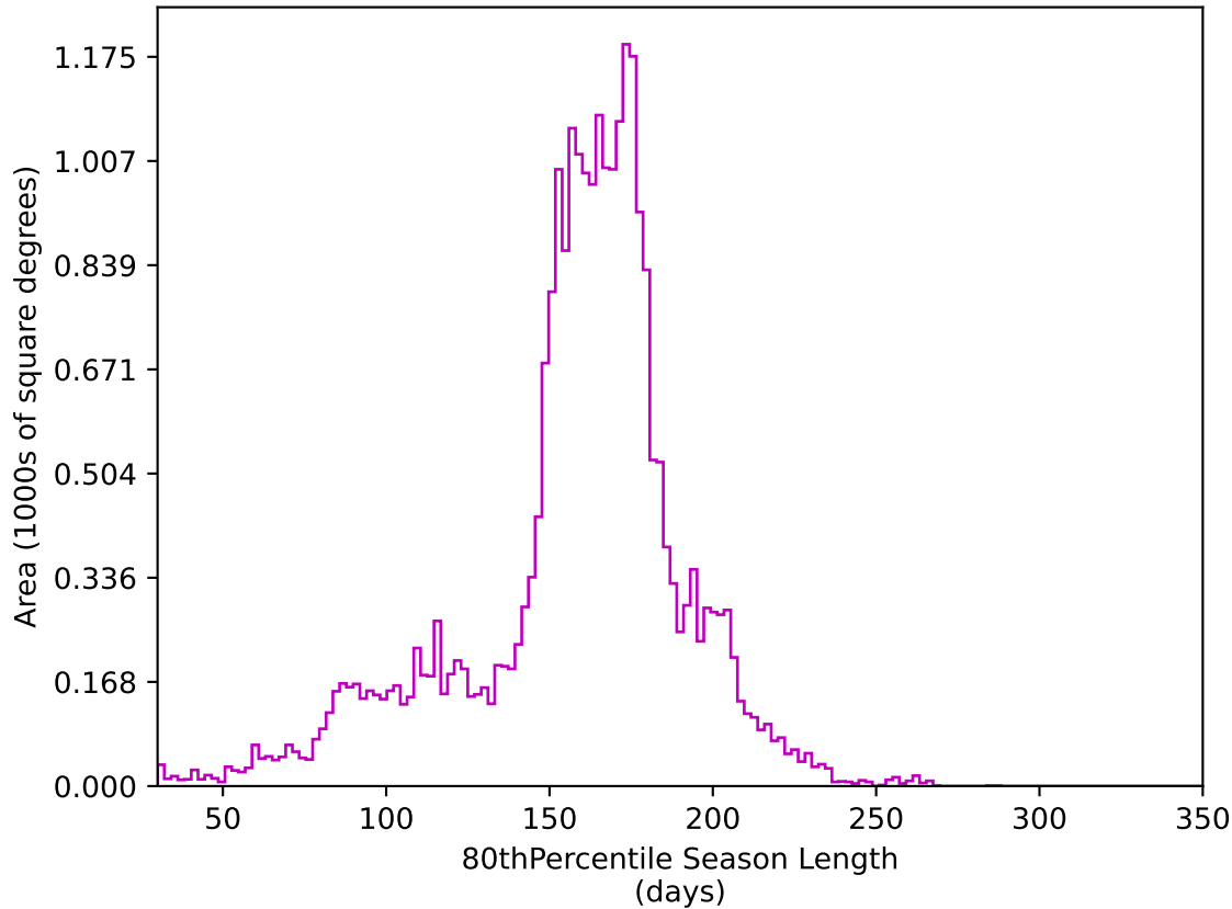
ddf_loaded_half_fl15_v3.4_10yrs All sky z band: 80thPercentile Season Length
