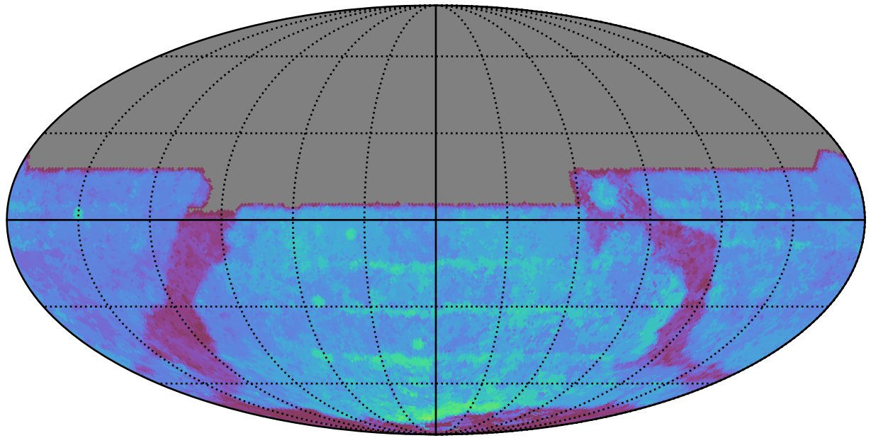
ddf_loaded_half_fl15_v3.4_10yrs All sky y band: 80thPercentile Season Length
