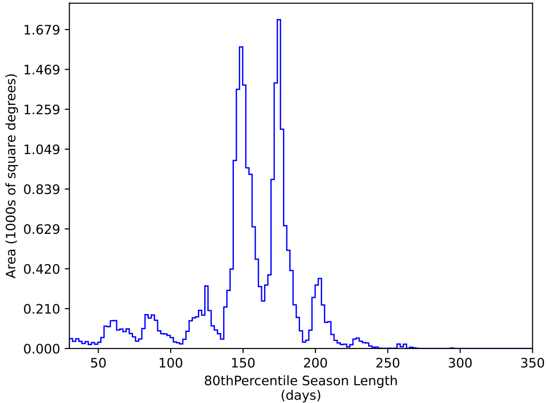
ddf_loaded_half_fl15_v3.4_10yrs All sky y band: 80thPercentile Season Length
