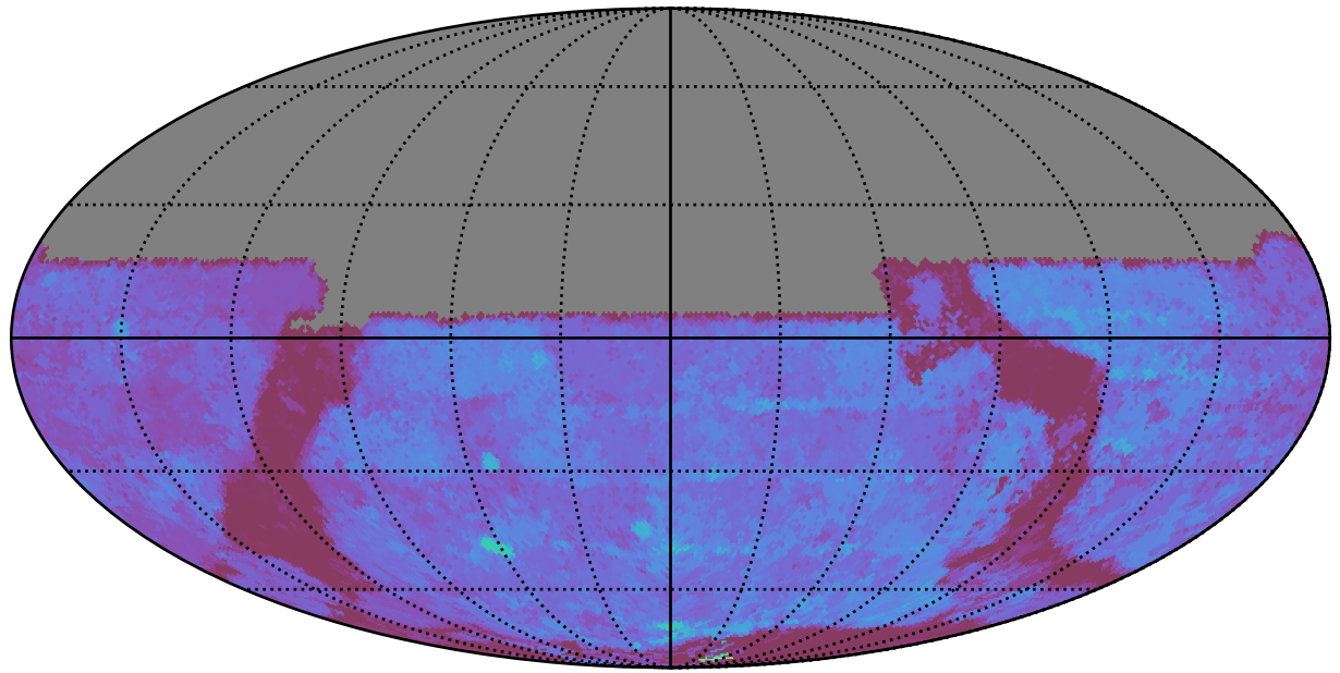
ddf_loaded_half_fl15_v3.4_10yrs All sky u band: 80thPercentile Season Length
