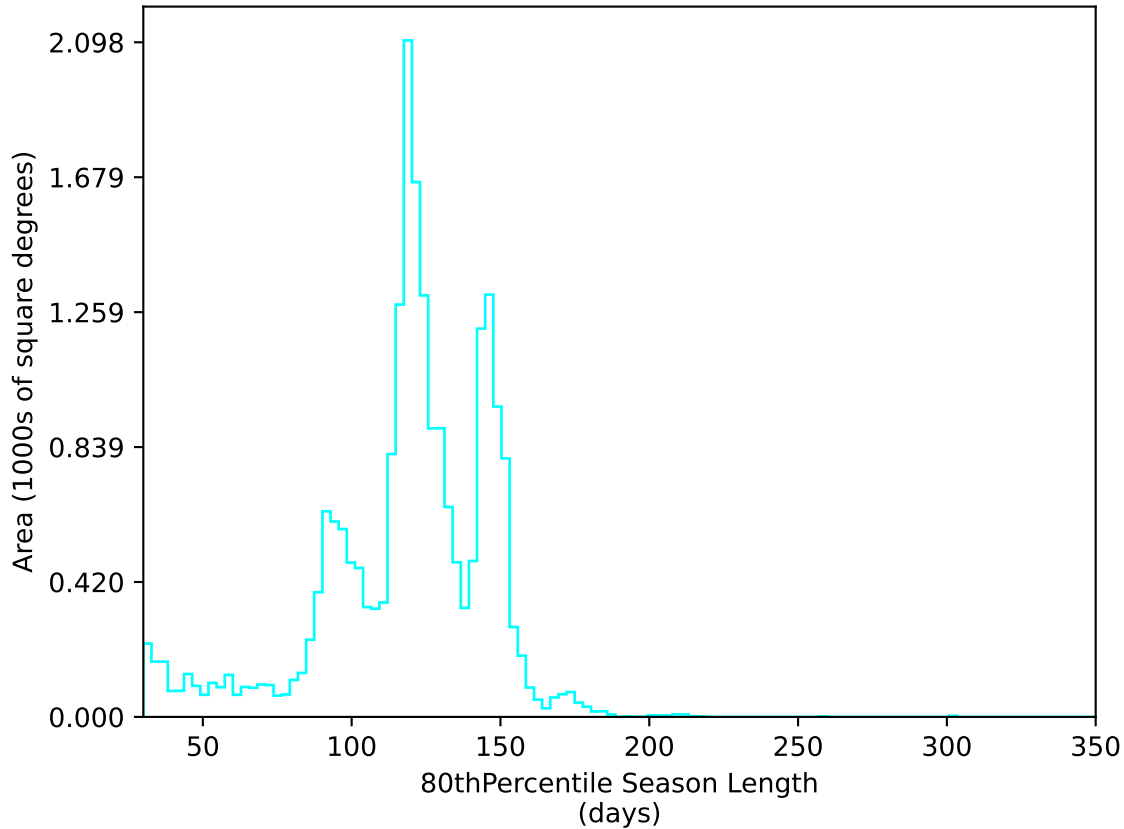
ddf_loaded_half_fl15_v3.4_10yrs All sky u band: 80thPercentile Season Length
