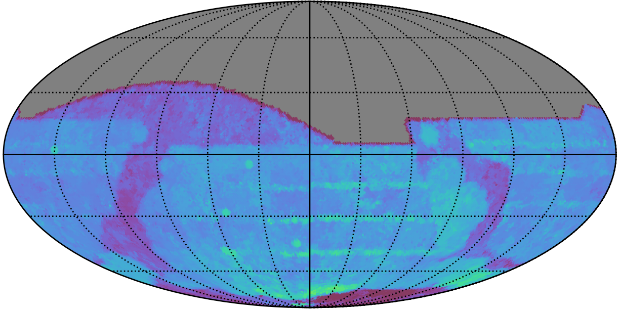
ddf_loaded_half_fl15_v3.4_10yrs All sky r band: 80thPercentile Season Length
