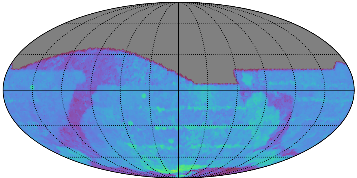
ddf_loaded_half_fl15_v3.4_10yrs All sky i band: 80thPercentile Season Length
