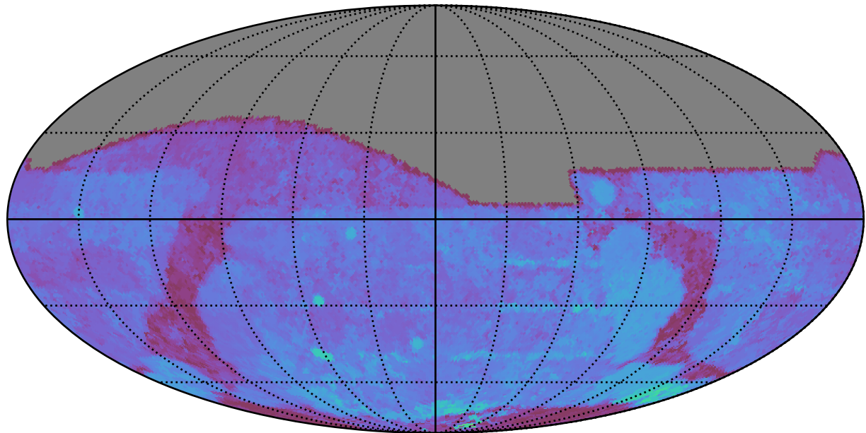
ddf_loaded_half_fl15_v3.4_10yrs All sky g band: 80thPercentile Season Length
