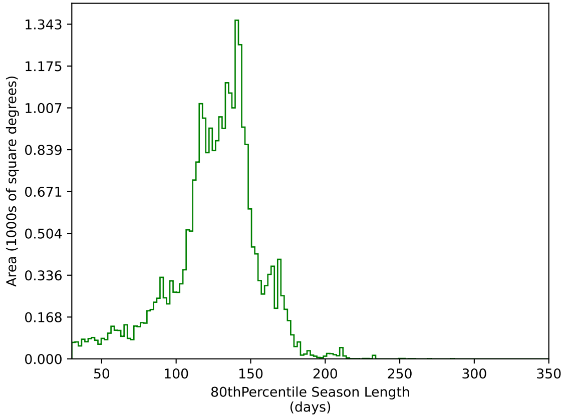
ddf_loaded_half_fl15_v3.4_10yrs All sky g band: 80thPercentile Season Length
