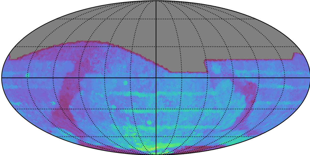
ddf_loaded_half_fl15_v3.4_10yrs All sky all bands: 80thPercentile Season Length
