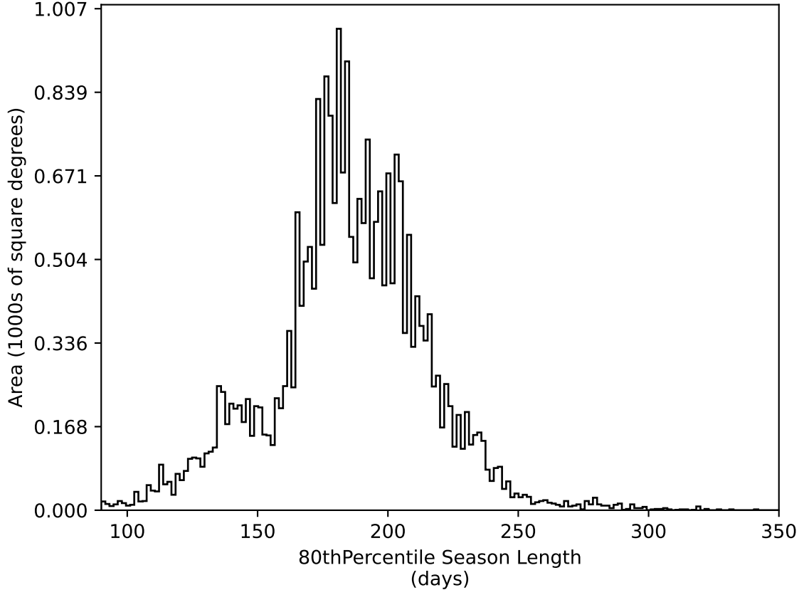
ddf_loaded_half_fl15_v3.4_10yrs All sky all bands: 80thPercentile Season Length
