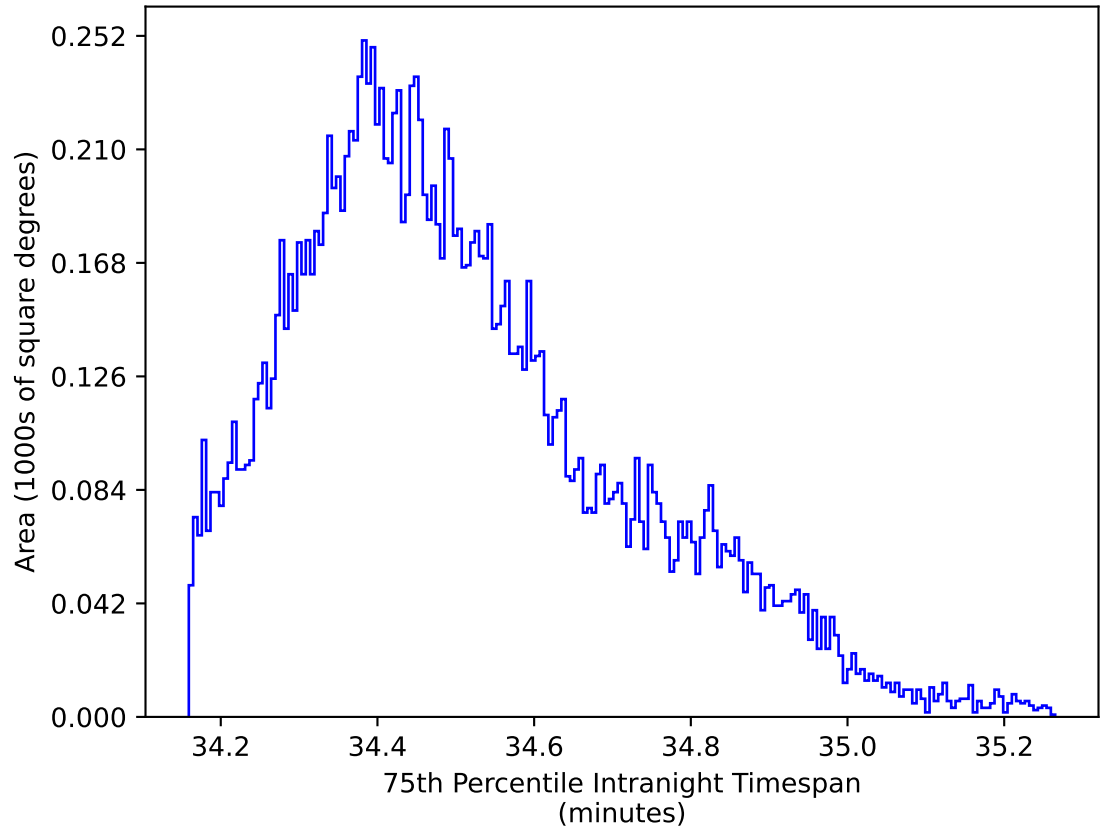
ddf_loaded_half_fl15_v3.4_10yrs WFD zy bands: 75th Percentile Intranight Timespan
